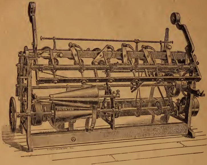
(SIX SPINDLE BALLER, 11 INCH GAUGE.)
